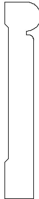
OB1020 5/8 X 3-3/8
