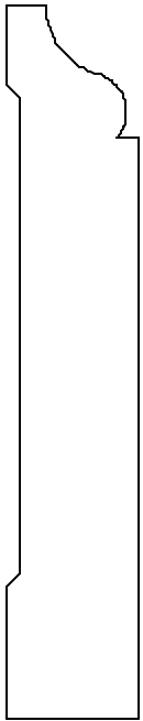
OB1001 5/8 X 3-3/8
