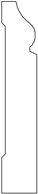
OB1029 5/8 X 3-3/8
