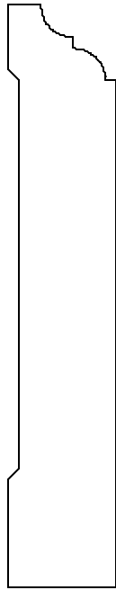
OB1079 5/8 X 3-3/8
