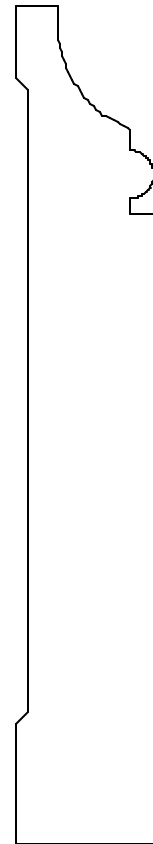
OB1054 3/4 X 4-3/8
