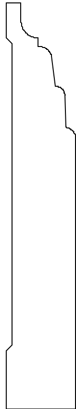
OB1067 3/4 X 4-3/8
