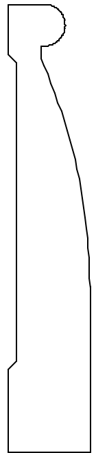
OB1021 5/8 X 3-3/8
