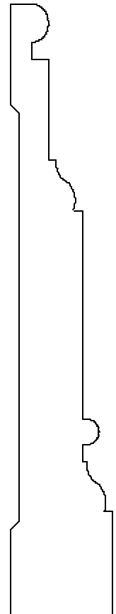
OB1090 3/4 X 4-1/2
