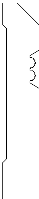
OB1045 5/8 X 3-3/8
