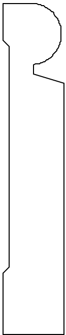
OB1015 5/8 X 3-3/8
