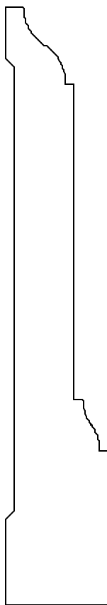
OB1050 3/4 X 4-3/8
