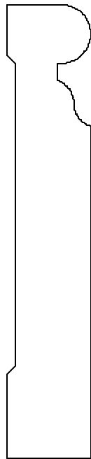
OB1017 5/8 X 3-3/8
