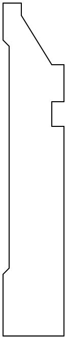
OB1043 5/8 X 3-3/8
