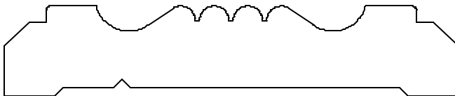
OB3418 11/16 X 3-3/8
